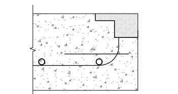
TYPICAL SAWCUT DETAIL
