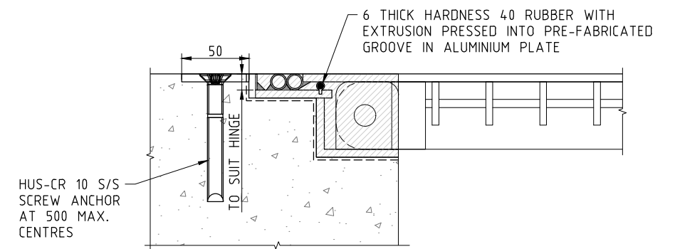
DETAIL S
