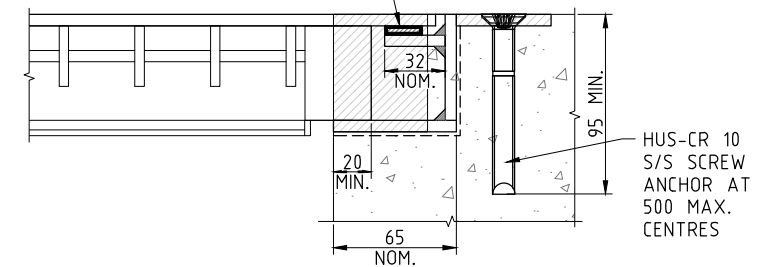
DETAIL T
