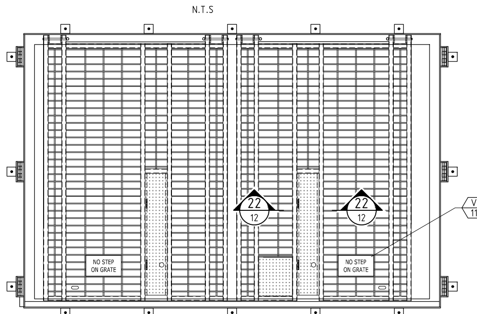
MULTIPLE SAFETY GRATE PLAN
