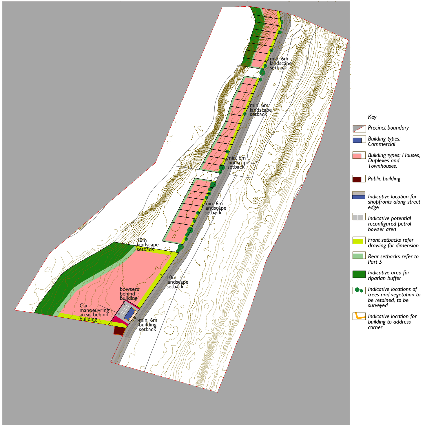
Figure 4.29 Control Diagram - South Tweed
