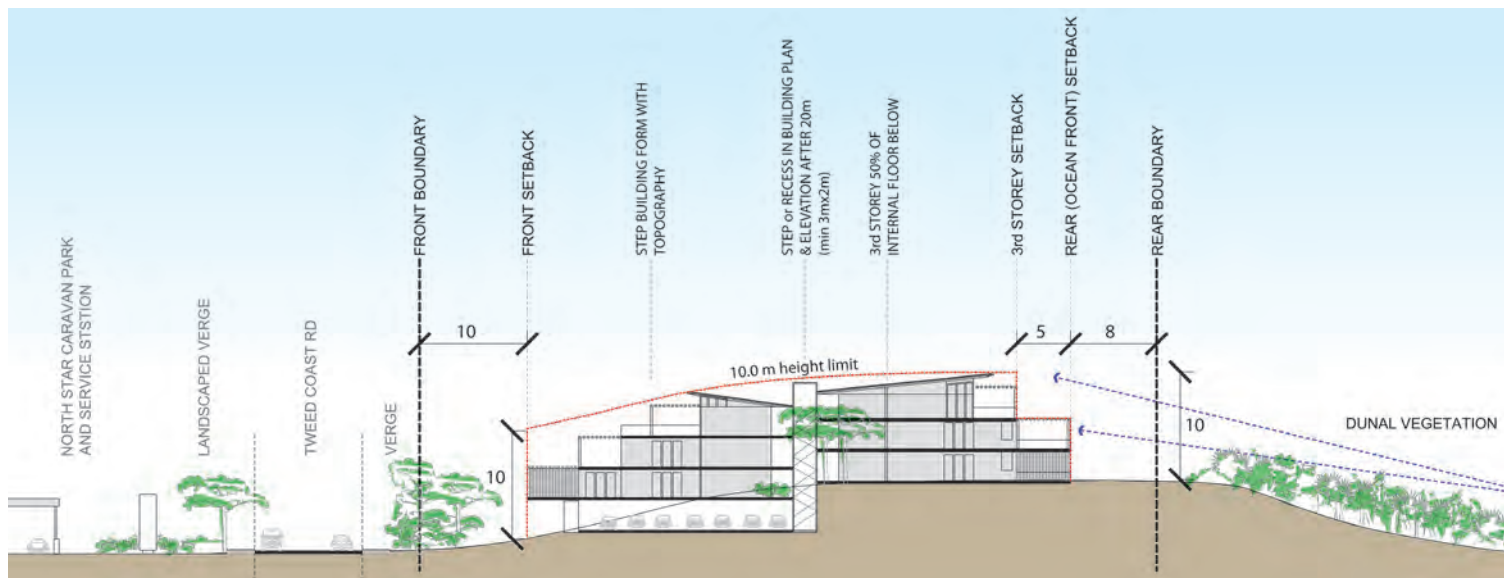
Figure 4.8 - Control Diagram - Indicative Section Height and Setback Controls
