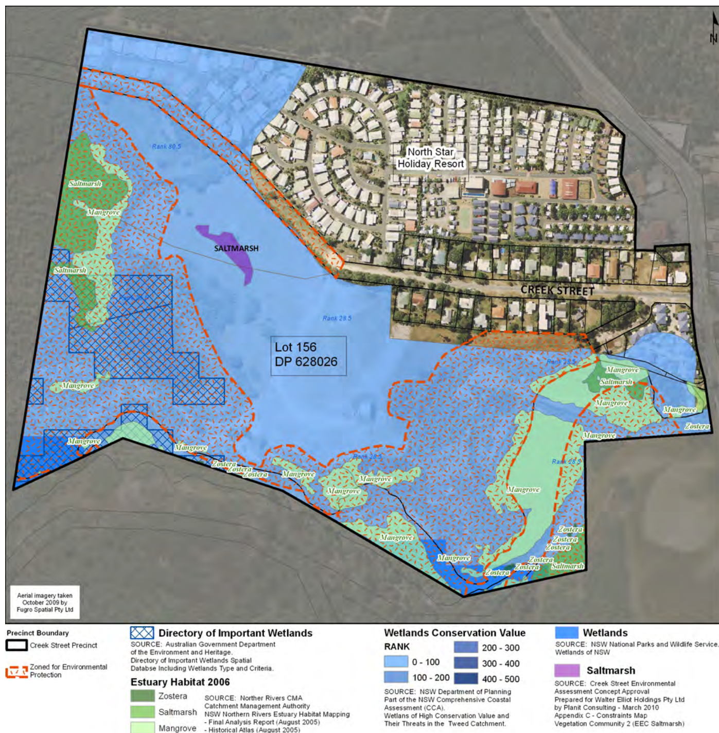
Figure 4.11 - Lot 156 Constraints Diagram
