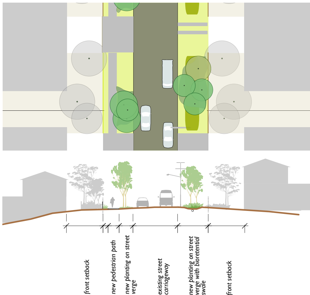
Figure 4.5 Indicative plan and section looking south along Peninsular Street
