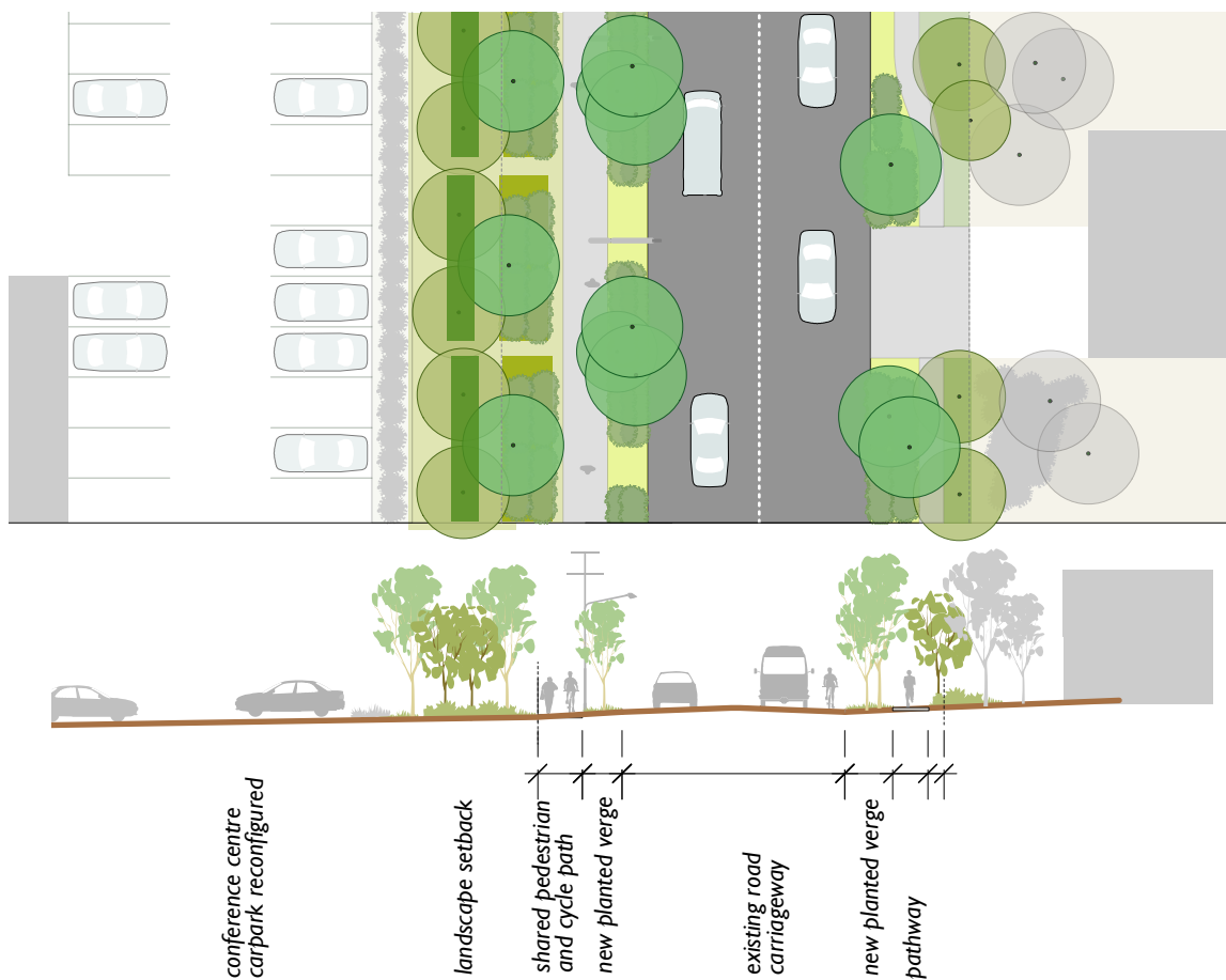
Figure 4.4 Indicative plan and section looking north from the northern star
