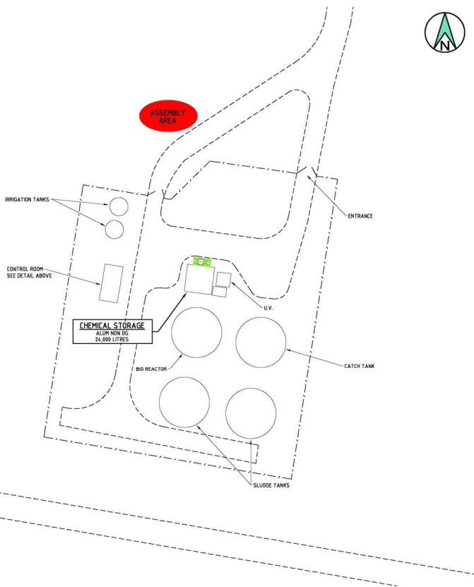
SITE PLAN
